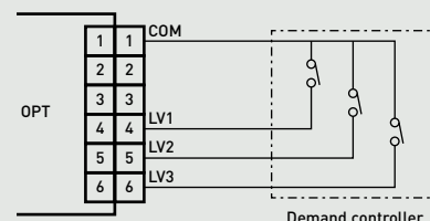
Indoor unit control PCB
