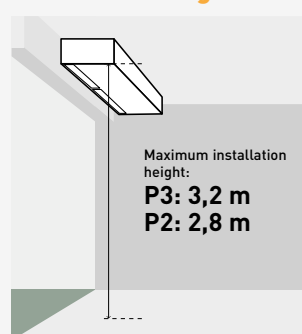
Suspended (standard)
