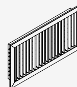
White aluminium supply grille with double row of adjustable fins (450 x 225 mm). For S-7110PQ41E.
