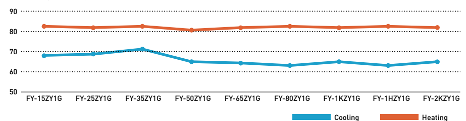
Heat exchange efficiency (%).
