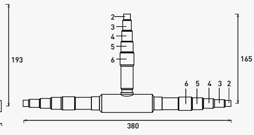
Liquid piping
