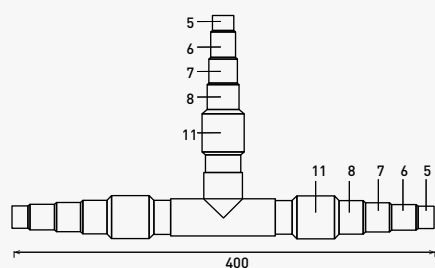
Suction piping
