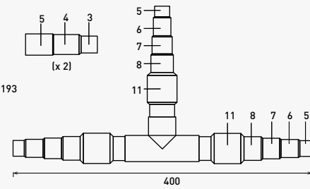
Discharge piping
