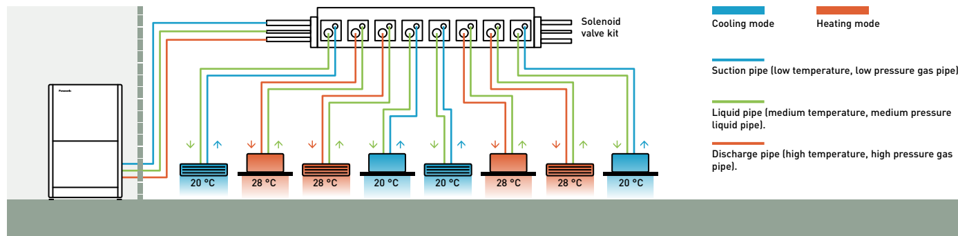
System structure.
