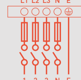
Three phase Power supply 3 x 400 V / 1 N ~ 50 Hz / **
