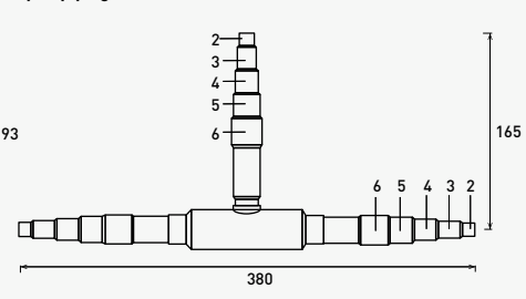
Liquid piping
