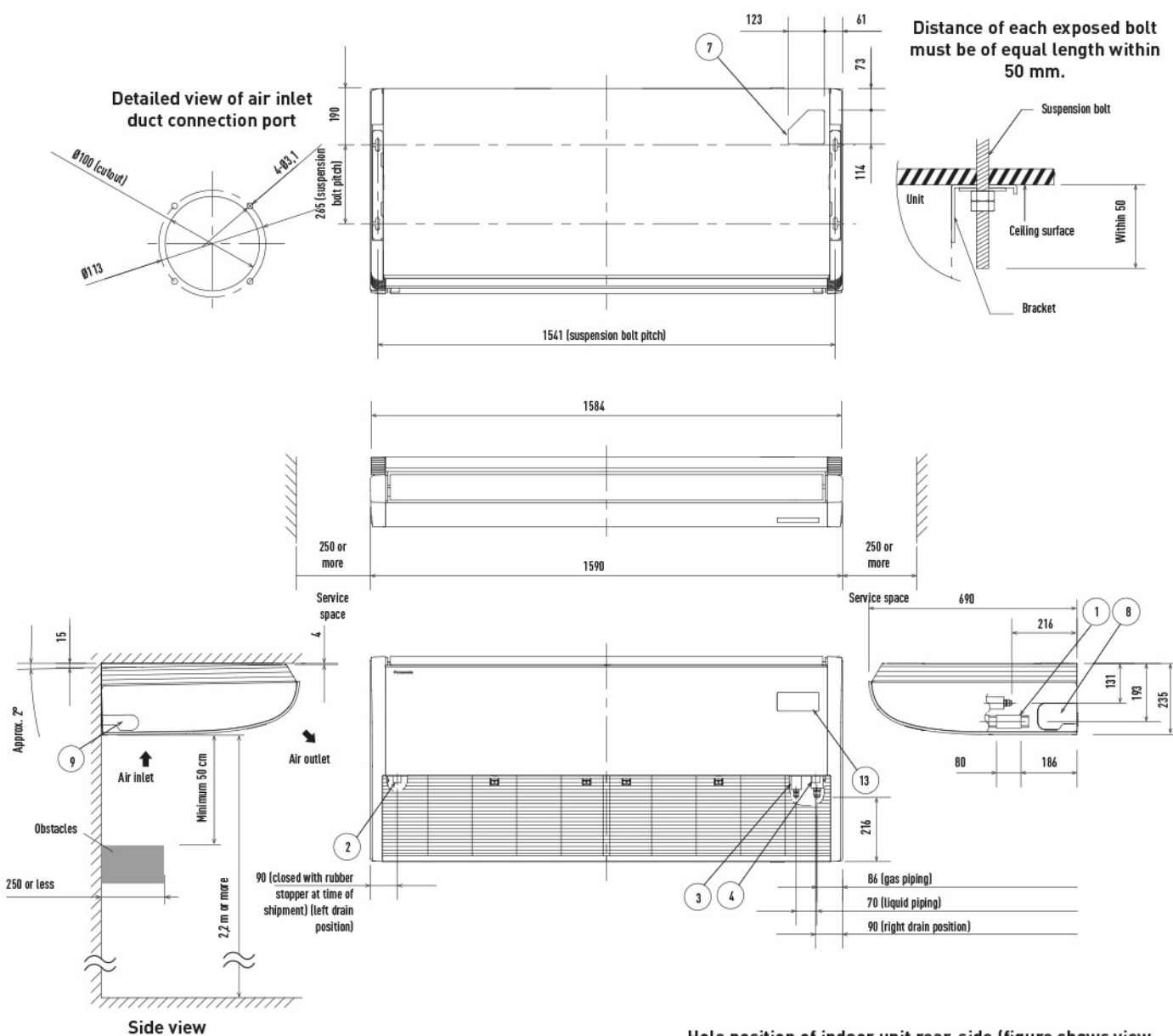
Hole position of indoor unit rear-side (figure shows view from front)
